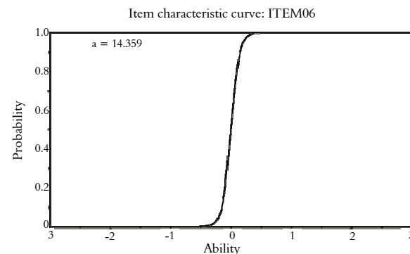
Figure 2. Characteristic curve of item 6 (existence of electrical energy).
