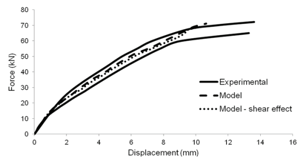
Figure 7. Numerical and experimental responses for 7\phi 10.0 mm beams.
