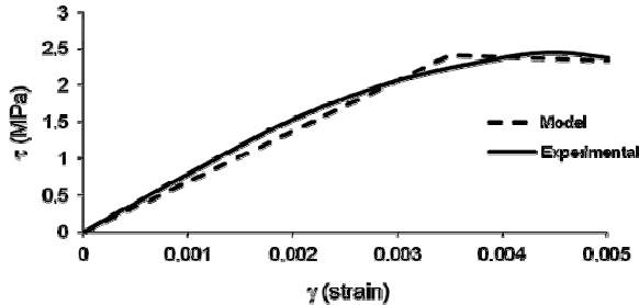
Figure 4. Parametric identification under pure shear.
