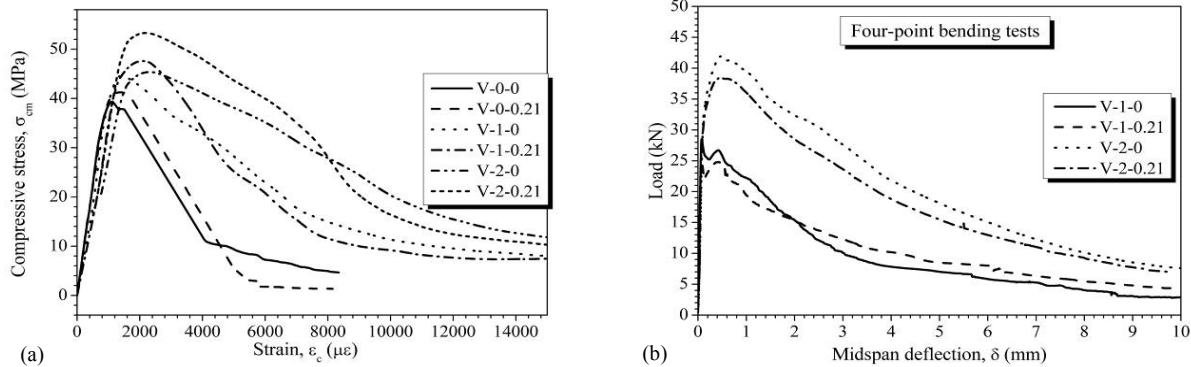
Figure 3. Average (a) compression test curve with displacement control and (b) four-point bending test on prismatic specimens.
