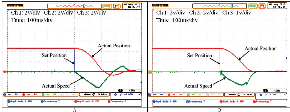
Figure 16. Reverse braking mode [180^\circ \text{ to } 0^\circ] : A. conventional PID controller response; B. fuzzy PID controller response.
