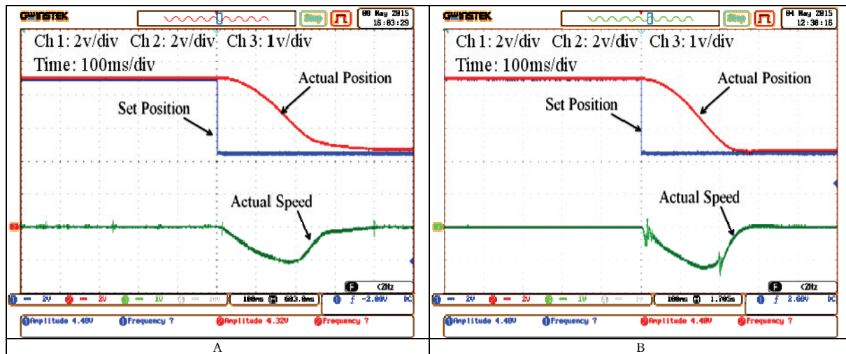
Figure 15. Reverse motoring mode [360^\circ \text{ to } 180^\circ] : A. conventional PID controller response; B. fuzzy PID controller response
