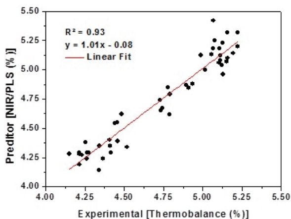
Figure 4. Comparison of predicted by NIR and measured by thermobalance results for moisture content in powdered egg.
