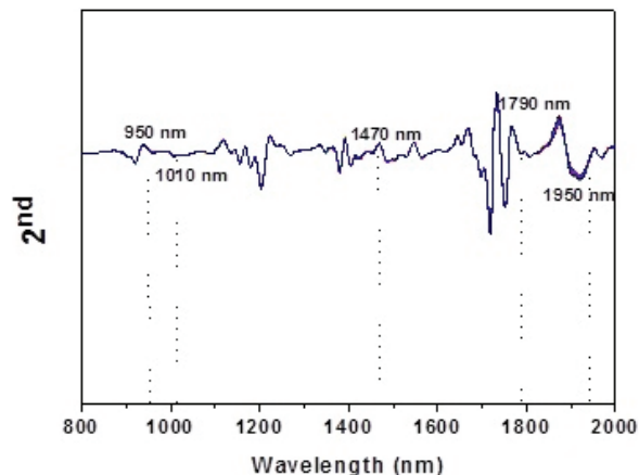
Figure 2. 2 nd Derivative spectra of 49 powdered egg samples with zoom in bands of O-H bonds.
