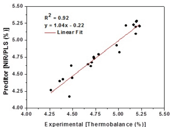
Figure 5. Powdered egg moisture content determined by thermobalance (X) related to predicted moisture given content by NIR applying PLS model (Y) (Model 1 – Table 3) for 21 unknown sample set of external validation.
