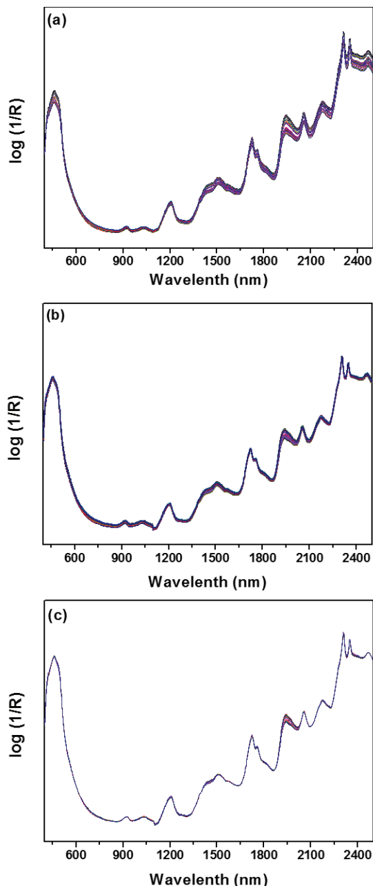
Figure 1. NIR spectra of 49 samples of powdered egg used to build the calibration curve; (a) Spectra without treatment; (b) Spectra with detrend, SNV and smooth treatments; (c) Spectra with detrend, MSC and smooth treatments.
