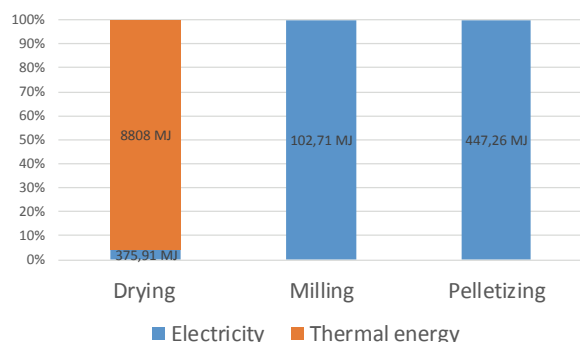
Figure 2. Energy consumption in the process.
