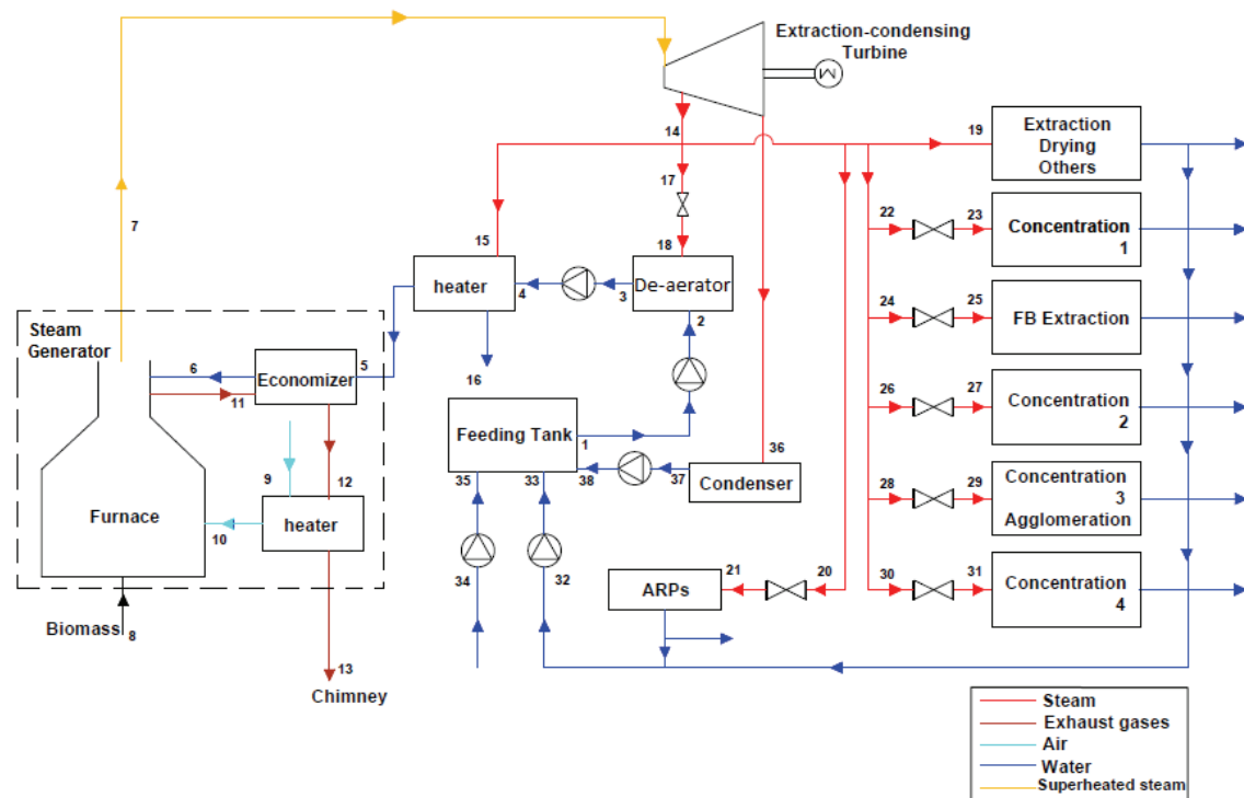
Figure 2. Trigeneration system.
