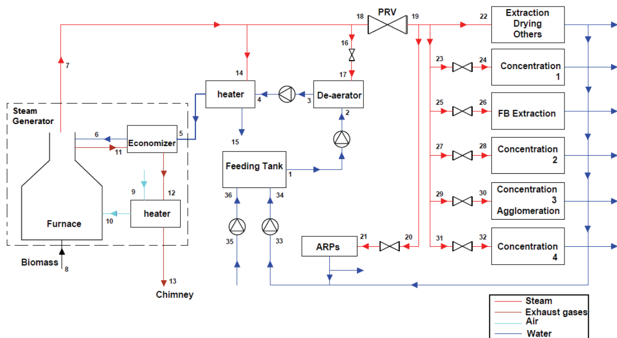
Figure 1. Current thermal system.
