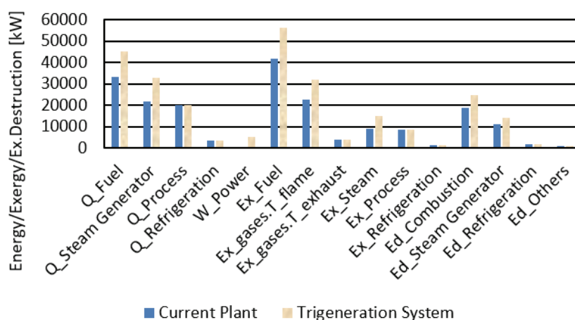
Figure 3. Energy, exergy and exergetic destruction in the current and trigeneration systems.
