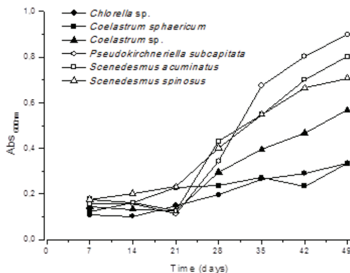
Figure 2. Growth kinetics of Chlorella sp., Pseudokirchneriella subcapitata , Coelastrum sp., Coelastrum sphaericum , Scenedesmus spinosus and Scenedesmus acuminatus in open ponds during 49 days.
