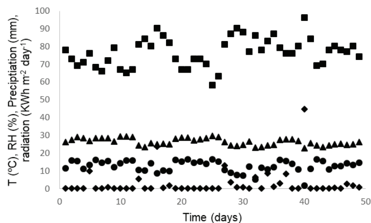
Figure 1. Meteorological data of (●) radiation ( \text{KWh m}^{-2}\text{ day}^{-1} ), (▲) temperature ( ^\circ\text{C} ), (◆) precipitation (mm) and (■) relative humidity (RH) (%) for the days corresponding to the cultivations in the open ponds.
