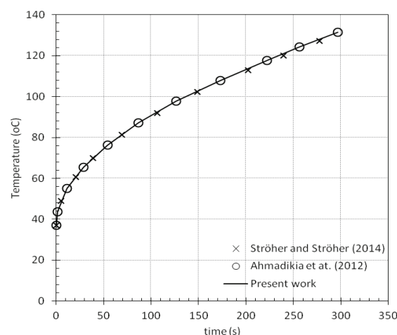
Figure 1. Skin surface temperature under constant heating boundary condition.
