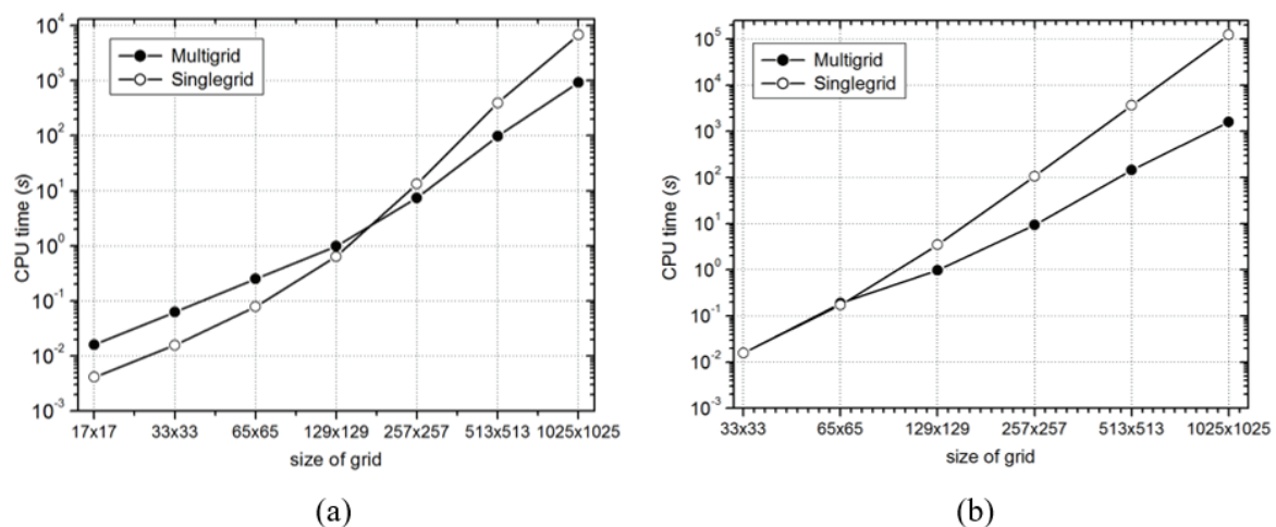
Figure 3. Analysis of the performance of the multigrid method, with refining of grid in transient and steady states, of heat conduction in human skin with melanoma (a) transient; (b) steady state.
