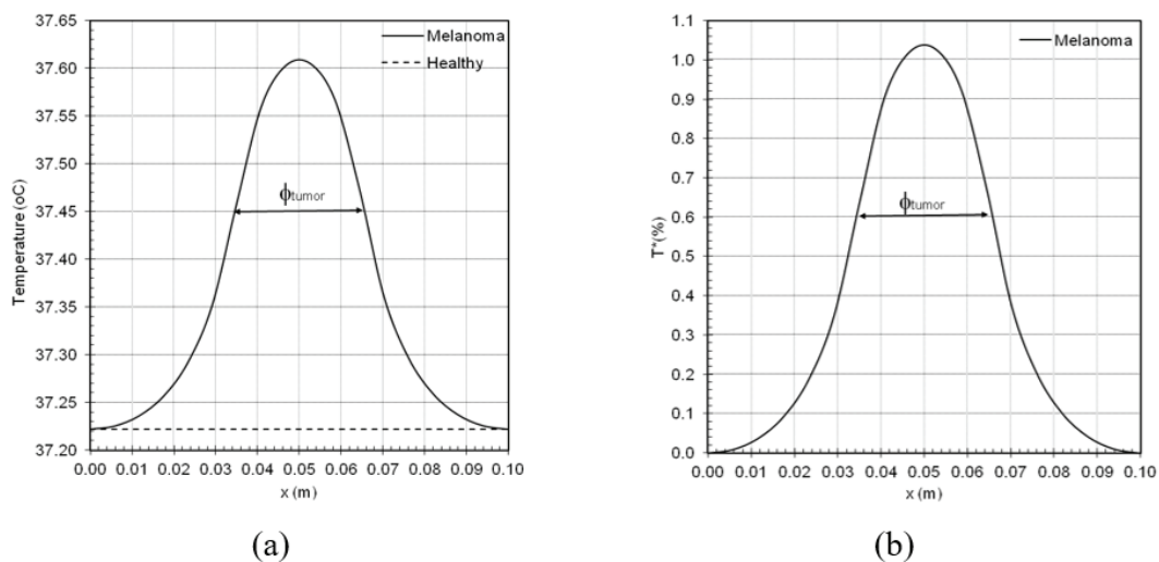
Figure 5. Temperature profile for healthy skin and skin with melanoma, \phi = diameter. (a) Increase of Temperature and (b) Increase of Dimensionless Temperature.
