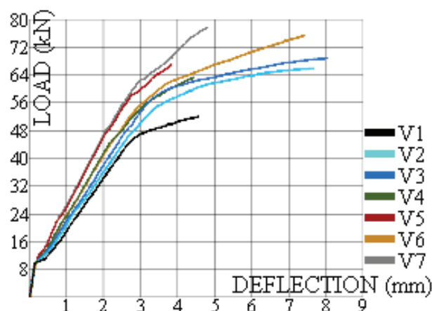
Figure 8. Load-deflection graph of the beams in the computational analysis. Source: Author.
