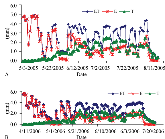
Figure 3. Evapotranspiration (ET), evaporation (E), and transpiration (T) of bean crop determined by the model during the experiments carried out in 2005 (A) and 2006 (B).
