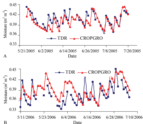
Figure 2. Variation of simulated and measured soil moisture at 20-cm depth during the experiment carried out in 2005 (A) and at 30 cm depth during the experiment conducted in 2006 (B).
