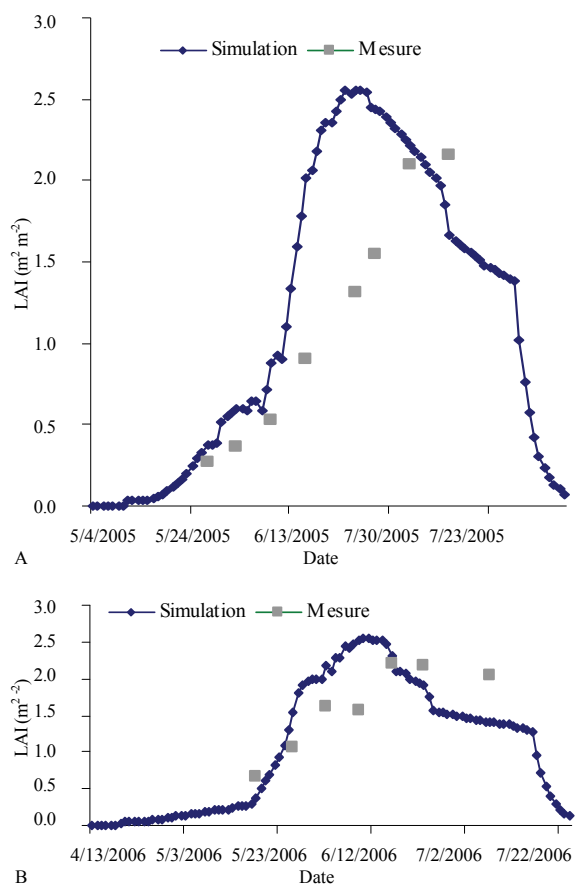
Figure 5. Leaf area indexes (LAI) determined in field and simulated by the model during the experiments carried out in 2005 (A) and 2006 (B).
