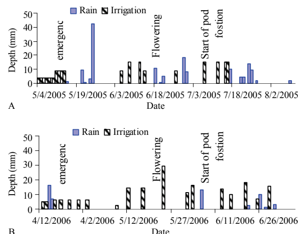
Figure 1. Rainfall and irrigation events during the experiments carried out in 2005 (A) and 2006 (B).
