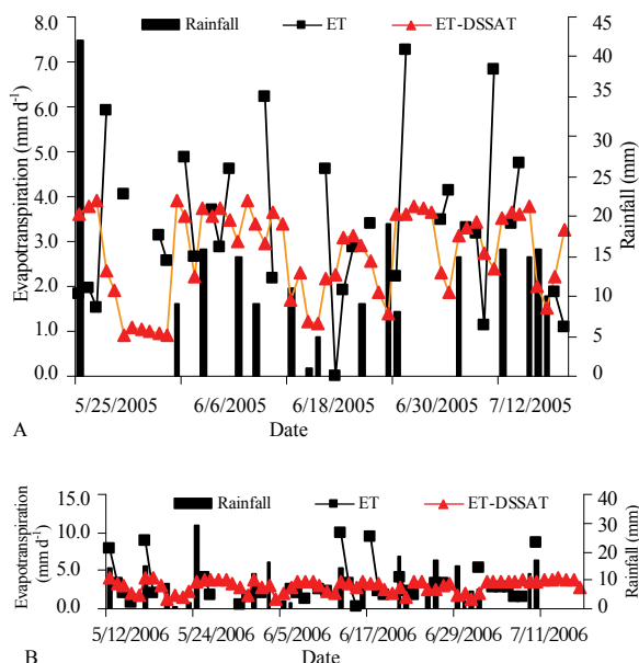
Figure 4. Evapotranspiration determined by the model and calculated from soil moisture values measured during the experiments carried out in 2005 (A) and 2006 (B).
