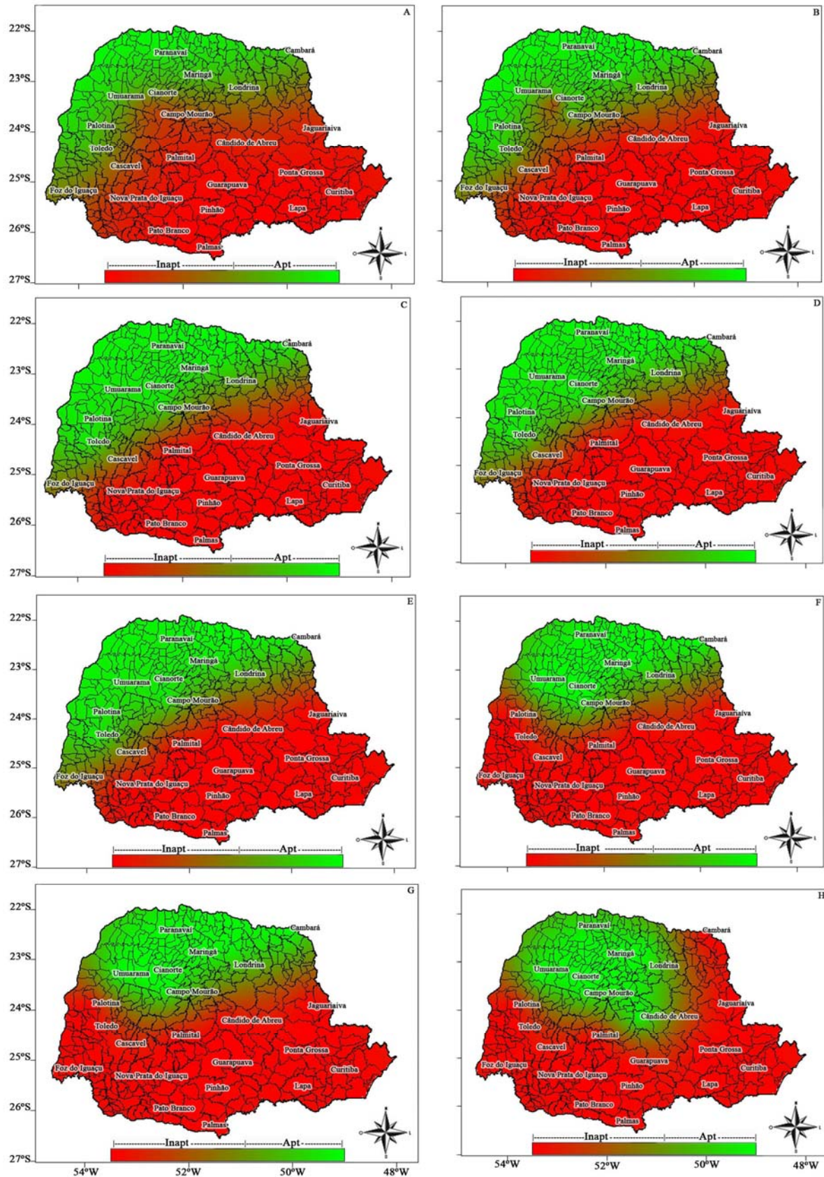
Figure 6. Suitability of the regions of Paraná State for undertaking sowing on 03/10 (A), 03/20 (B), 03/30 (C), 04/10 (D), 04/20 (E), 04/30 (F), 05/10 (G), and 05/20 (H).
