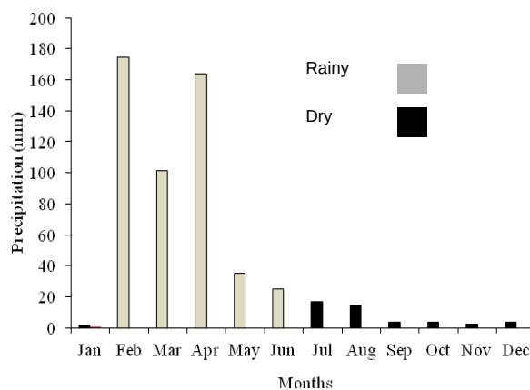
Figure 1. Monthly precipitation recorded in 2007, in Taperoá, Paraíba State (AES, 2008).
