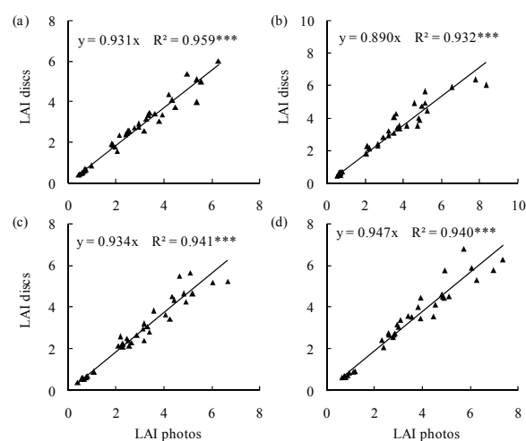
Figure 2. Relationship between the leaf area index (LAI) estimated by the digital photo method (photos) and by the leaf disc method (discs) in four soybean cultivars, including (a) BMX Apolo® RR, (b) BRS 284®, (c) BMX Energia® RR and (d) FPS Urano® RR in the 2010/2011 growing season in Guarapuava, Paraná State. ***: Statistically significant at 0.1%.
