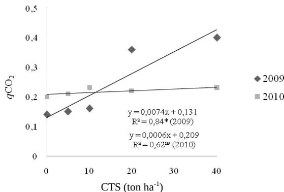
Figure 5. Soil respiratory quotient ( q\text{CO}_2 ) in soil after two years of CTS amendment. ns – no significant, * – significant p < 0.05 .
