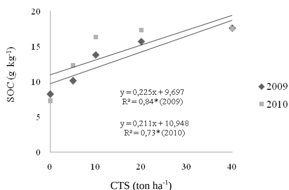
Figure 1. Soil organic C (SOC) in soil after two years of CTS amendment. ns - no significant; * - significant p < 0.05 .
