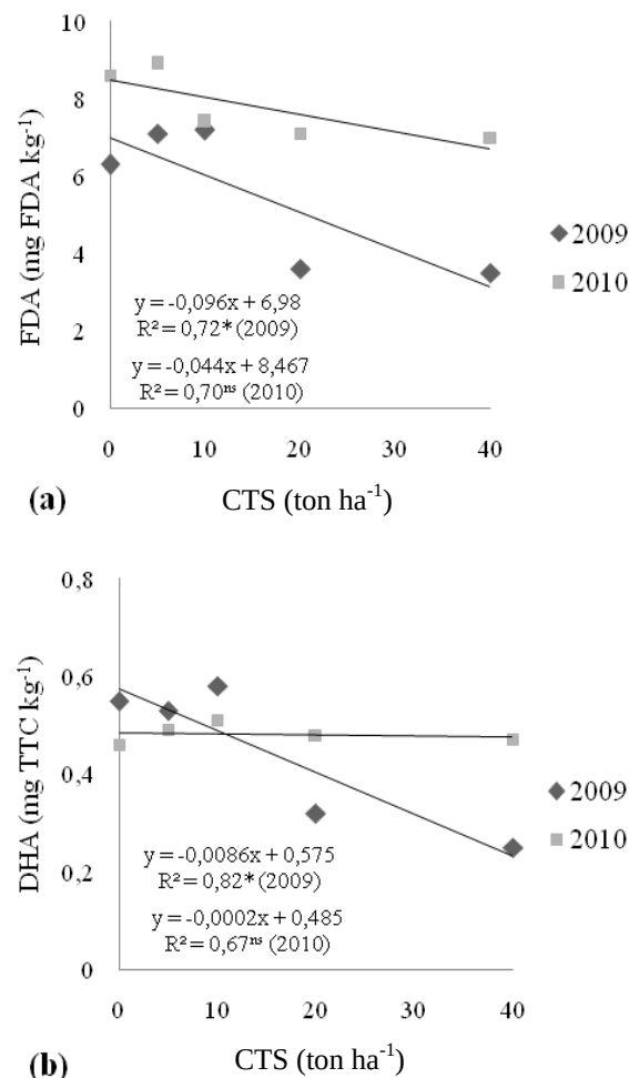
Figure 4. Fluorescein diacetate hydrolysis (FDA) (a) and dehydrogenase activity (DHA) (b) in soil after two years of CTS amendment. ns – no significant, * – significant p < 0.05 .
