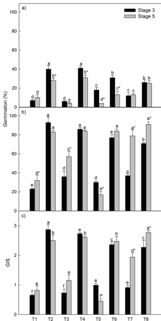
Figure 3. a) Germination rates at 14 days after sowing and b) 30 days after sowing, c) Germination Index Speed (GIS) obtained in seeds at maturity stages 3 and 5. T1: (CEPA (0 mol dm -3 ) + GA 3 (0 mg dm -3 ) + KN 3 (0 mol dm -3 ); T2: (CEPA (0 mol dm -3 ) + GA 3 (0 mg dm -3 ) + KN 3 (1 mol dm -3 ); T3: (CEPA (0 mol dm -3 ) + GA 3 (50 mg dm -3 ) + KN 3 (0 mol dm -3 ); T4: (CEPA (0 mol dm -3 ) + GA 3 (50 mg dm -3 ) + KN 3 (1 mol dm -3 ); T5: (CEPA (5x10 -7 mol dm -3 ) + GA 3 (0 mg dm -3 ) + KN 3 (0 mol dm -3 ); T6: (CEPA (5x10 -7 mol dm -3 ) + GA 3 (0 mg dm -3 ) + KN 3 (1 mol dm -3 ); T7: (CEPA (5x10 -7 mol dm -3 ) + GA 3 (50 mg dm -3 ) + KN 3 (0 mol dm -3 ); T8: (CEPA (5x10 -7 mol dm -3 ) + GA 3 (50 mg dm -3 ) + KN 3 (1 mol dm -3 ). Means followed by same letter do not differ significantly from one another (Scott-Knott test, p ≤ 0.05). *Denotes differences between seeds at stages 3 and 5 only within each treatment (a pair of rectangles) (F-test, p ≤ 0.05). n = 4 ± SE.
