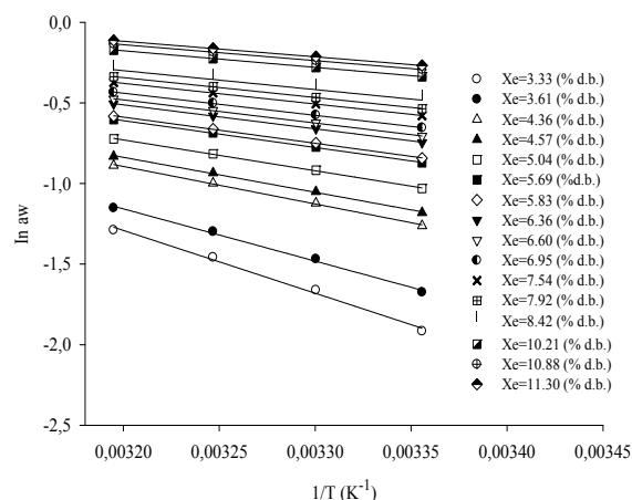
Figure 1. Curves of the neperian logarithm of the water activity (decimal) for specific values of equilibrium moisture content (% d.b.) as a function of the values of 1/T (K -1 ) for forage turnip seeds.
