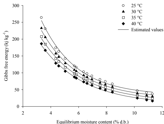
Figure 3. Gibbs free energy as a function of the equilibrium moisture content of forage turnip seeds.
