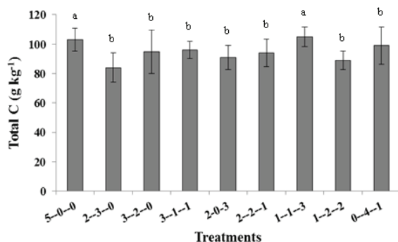
Figure 2. Total carbon in the biofertilizers with different proportions of the 3 types of organic matter (sugarcane mud cake: earthworm compost: crop residue), inoculated with the selected diazotrophic bacteria Beijerinckia indica (strain NFB 10001), after
