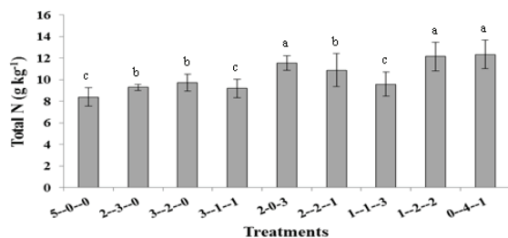
Figure 1. Total N in the biofertilizers with different proportions of the 3 types of organic matter (sugarcane mud cake: earthworm compost: crop residue), inoculated with selected diazotrophic bacteria Beijerinckia indica (strain NFB 10001), during the maturation phase under various incubation times (0, 10, 20, 30, and 40 days) at room temperature (28 ± 2°C).
