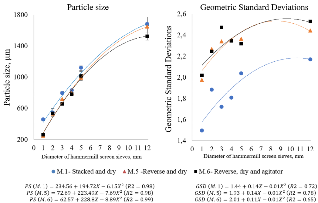
Figure 1. Particle size and geometric standard deviations of corn ground by different features of the hammermill screen sieves (FS) analyzed under different sieving methodologies.
