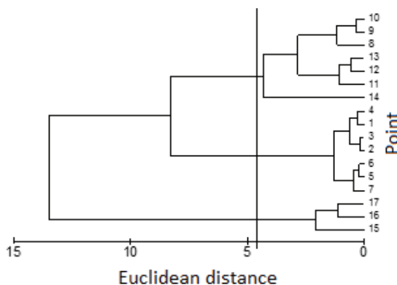
Figure 2. Dendrogram of the cluster analysis for distances between sampling sites and mouths of the Paranaguá Estuarine Complex.
