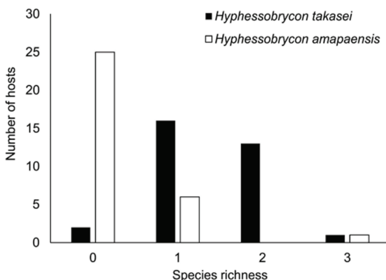
Figure 2. Species richness of parasites in Hyphessobrycon takasei and H. amapaensis from the State of Amapá, Brazil.
