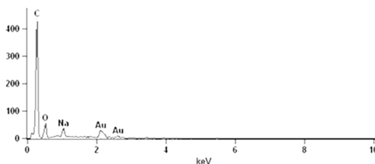
Figure 4. EDS spectrum of IO material.
