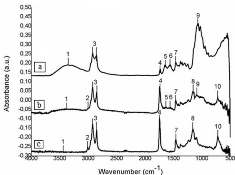
Figure 2. FTIR spectra (ATR). a) Chitosan; b) IO; and c) NIO.
