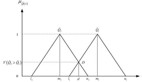
Figure 2: The intersection between \tilde{Q}_1 and \tilde{Q}_2 .
