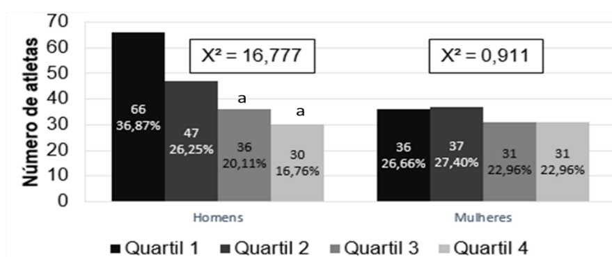
Figure 1. Distribution of the birth quartiles of the male and female athletes ranked for the 2016/17 Super Leagues.
