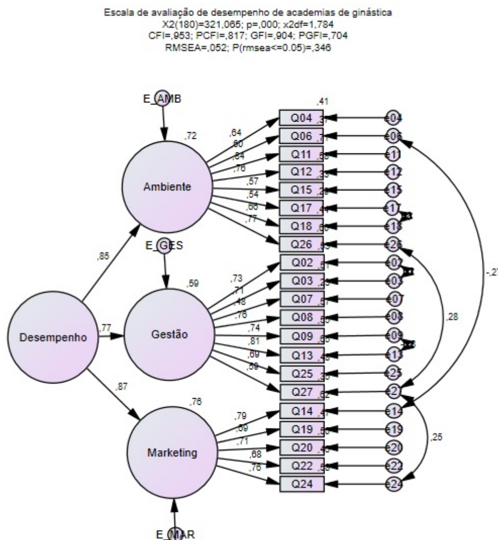
Figure 3. Second-order Confirmatory Factor Analysis of the evaluation on Quality of Services Provided by Gyms construct
